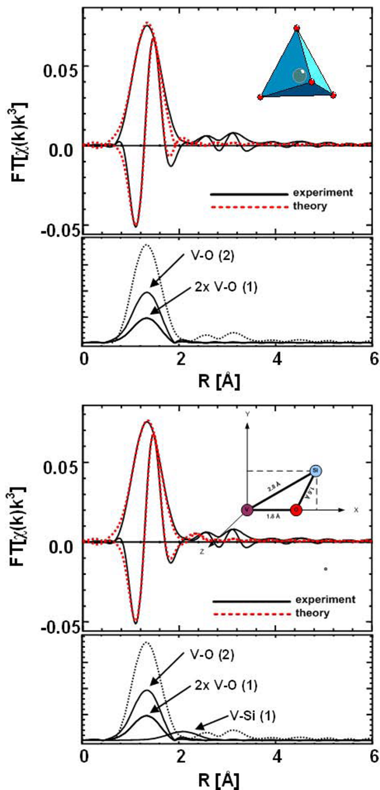
Figure 5 Experimental (solid) V K edge FT[\chi(k)k^3] of dehydrated V_xO_y/SBA-15 (10.8 wt %) together with theoretical XAFS functions (top: "isolated VO_4 " model, bottom: addition of V-Si path to "isolated VO_4 " model). Insets show the VO_4 tetrahedron (top) and a schematic representation of the V-Si path employed (bottom). Also shown are the Fourier transformed \chi(k)k^3 of the individual scattering paths together with corresponding coordination number in.
